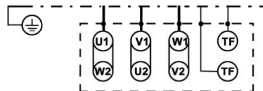
Delta-connection
