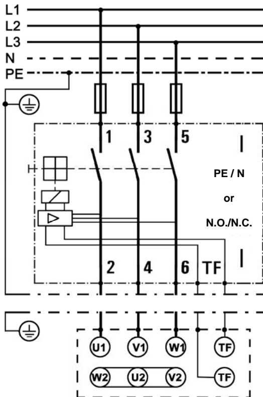
Star-connection
